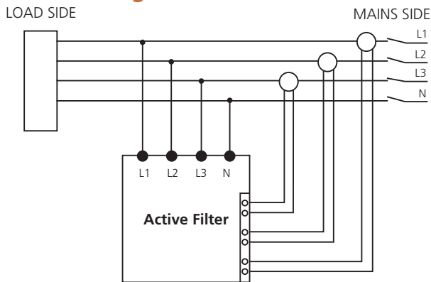
Close Loop Connection
